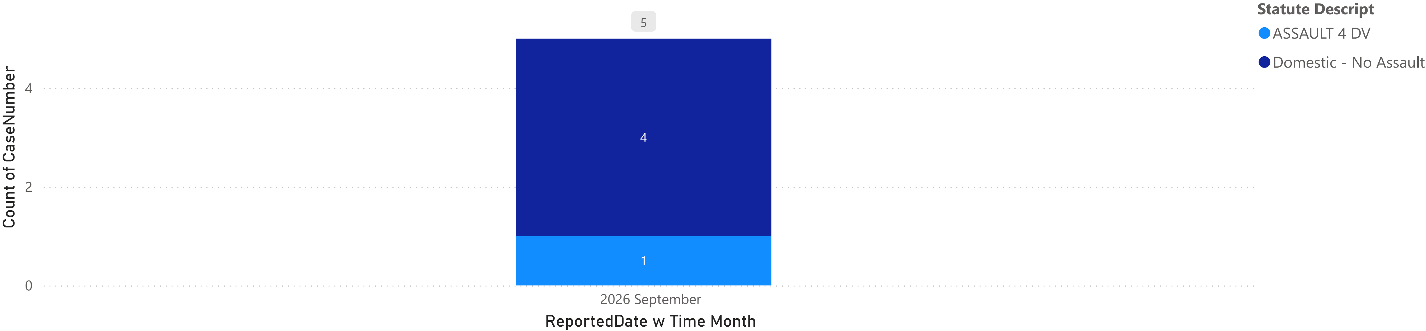
Count of Statute (*) Case Number
